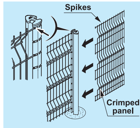
5 - Insert the second panel. Repeat operation. Once installation is complete, remove the AXIS tension blocks or the AXOR wedges (reusable).
