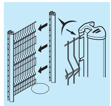
3 - Insert the second post into the panel.
